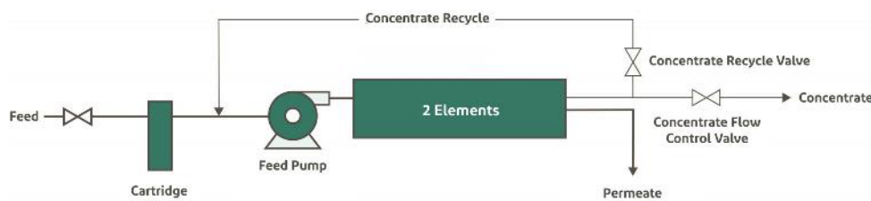
Figure 31: Single-module system
