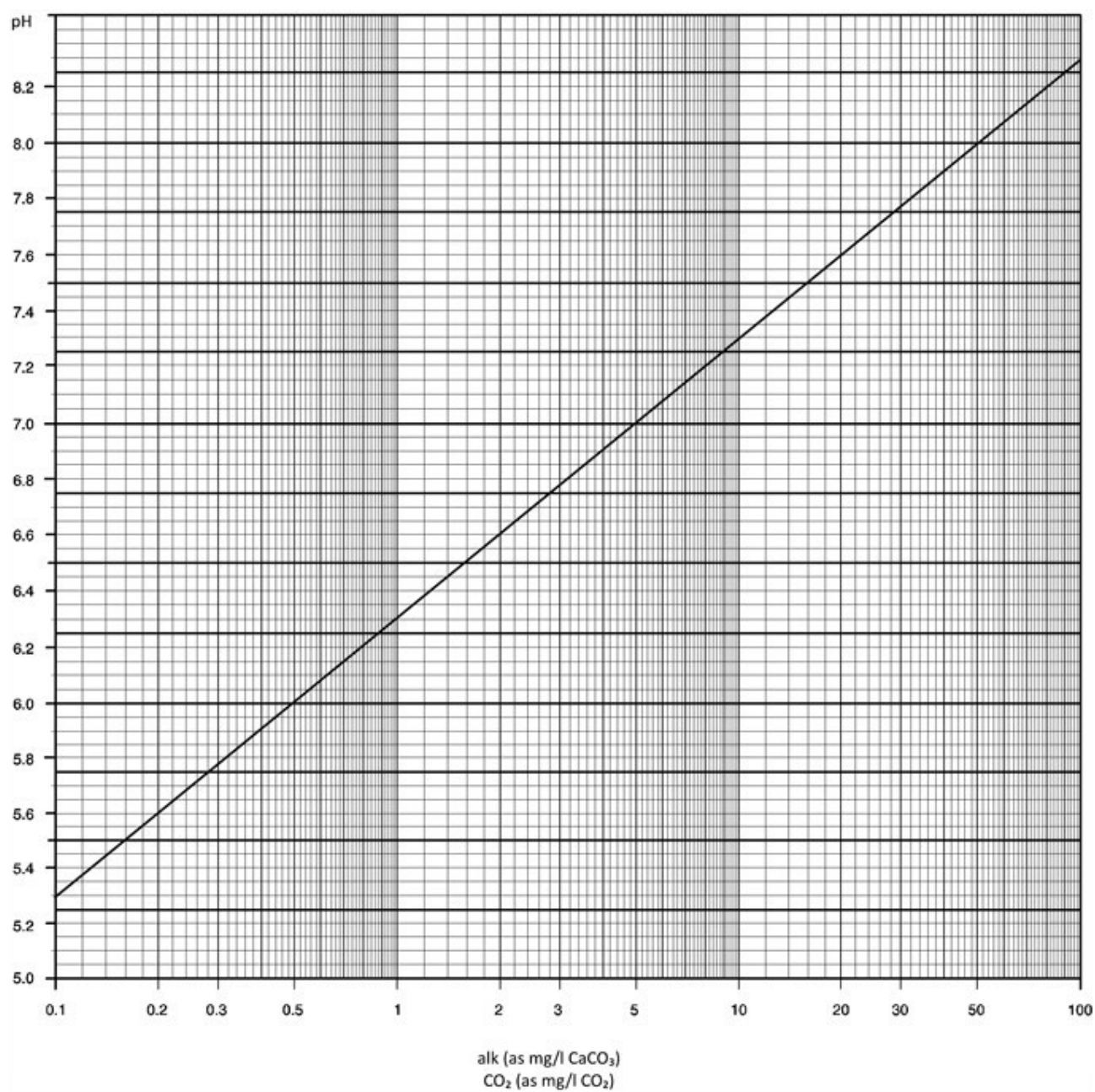
Figure 17: pH versus methyl orange alkalinity/free \text{CO}_2
