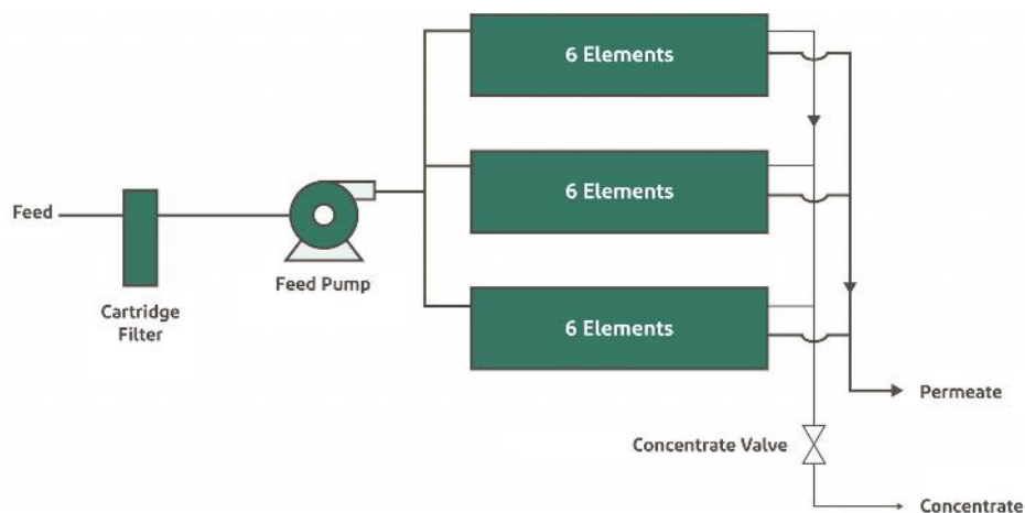
Figure 32: Single-stage system
