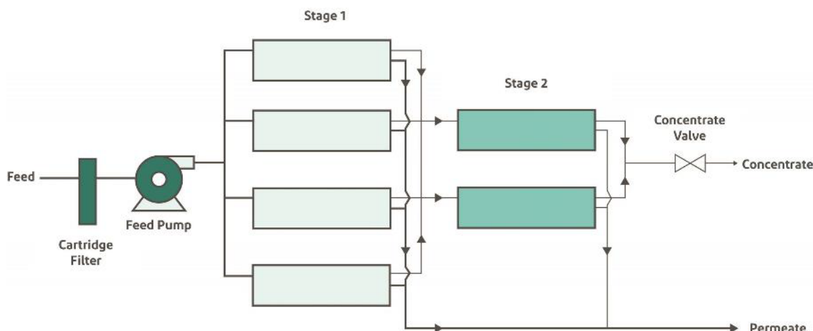
Figure 33: Two-stage system
